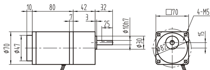
调速电机 Speed Control Motors 3IK15GN-□R+3GN□K
