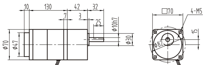
调速电磁制动电机 Speed Control & brake Motors 3IK15GN-□MR+3GN□K
