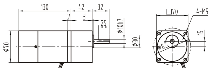
调速电磁制动电机 Speed Control & brake Motors 3IK15GN-□MR+3GN□K
