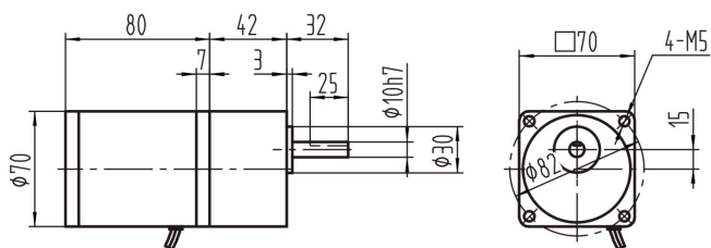
调速电机 Speed Control Motors 3IK15GN-□R+3GN□K
