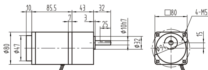
调速电机 Speed Control Motors 4IK25GN-□R+4GN□K
